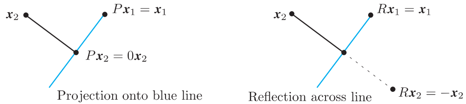
Figure 6.2: Projections P have eigenvalues 1 and 0. Reflections R have \lambda = 1 and -1 . A typical \mathbf{x} changes direction, but not the eigenvectors \mathbf{x}_1 and \mathbf{x}_2 .
