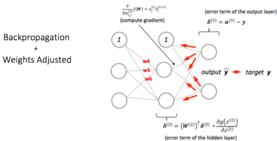
Figure 6: backward propagation and weight updation step in a multi layer perceptron
