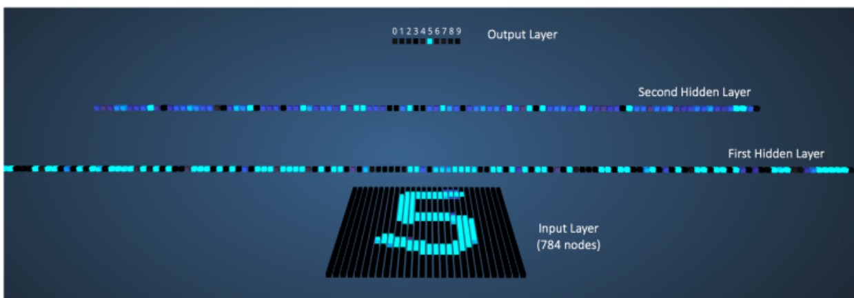
Figure 8: visualizing the network for an input of '5'
